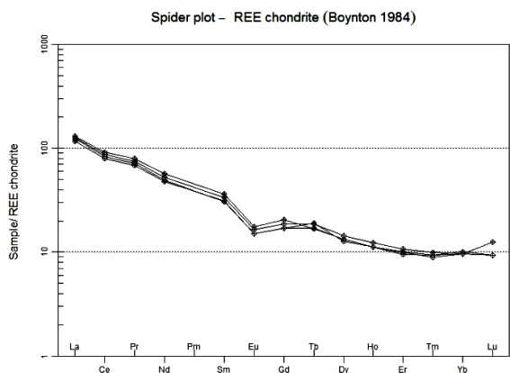
Fig. 10. REE pattern of Se-Chahun rhyolite rocks (Boynnton, 1984).
