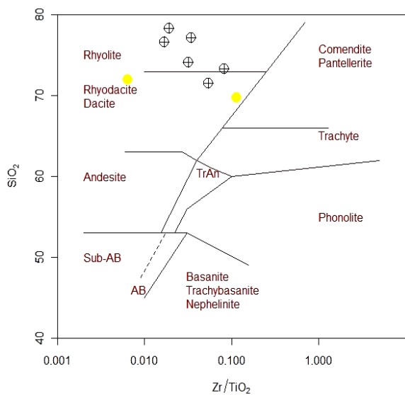
Fig. 7. Classification of rhyolite rocks (Winchester & Floyd, 1977).
