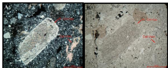
Fig. 4. Photmicrographs of plagioclase phenocryst in rhyolite rocks (A, XPL and B, PPL).
