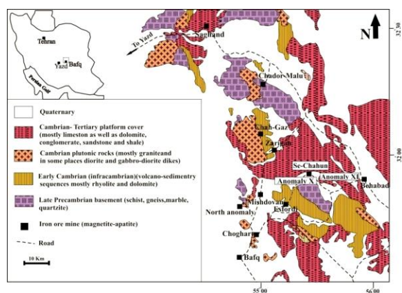
Fig. 1. Simplified geological map of the Bafq mining district and location Se-Chahun ore deposits and igneous rocks (Modified from Torab, 2008).
