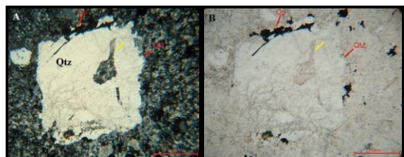
Fig. 3. Photmicrographs of quartz phenocryst in Se-Chahun rhyolites, (A, XPL and B, PPL).
