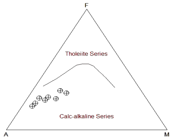
Fig. 8. Discriminant diagram between tholeiitic, calcalkaline series of rhyolite rocks of the Se-Chahun district (Irvine & Baragar, 1971).
