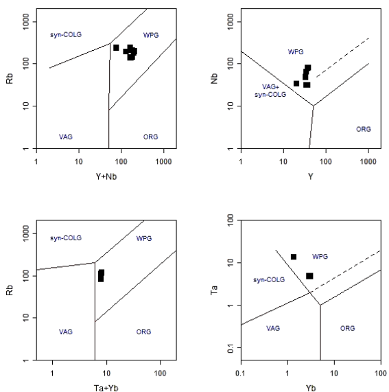
Fig. 11. Graph partitioning the tectonic rhyolite rocks (Pierce et al. , 1984).
