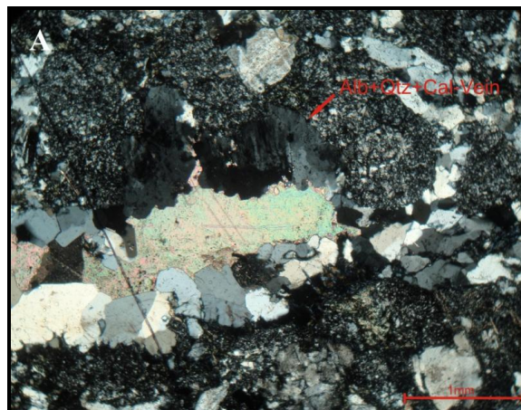
Fig. 5. Photmicrographs of Quartz veins with calcite in Se-Chahun rhyolites.
