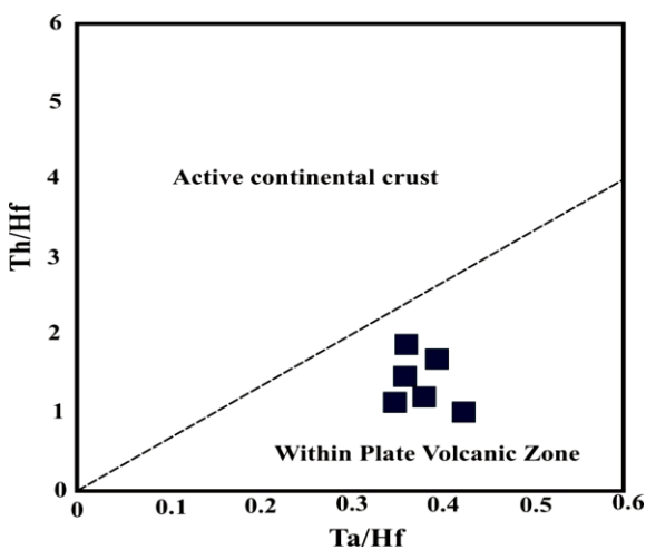
Fig. 12. Tectonic diagrams (Schandl and Gorton, 2002).
