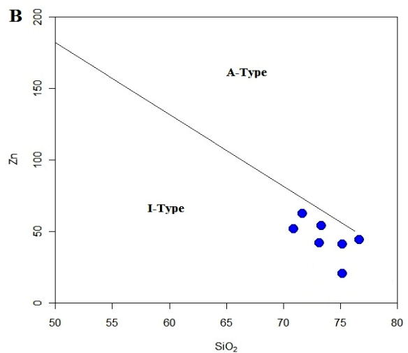
Fig 9. A- Diagram Zr versus \text{SiO}_2 and B- Zn versus \text{SiO}_2 (Collins et al . 1982). All samples plotted in the I-type area.
