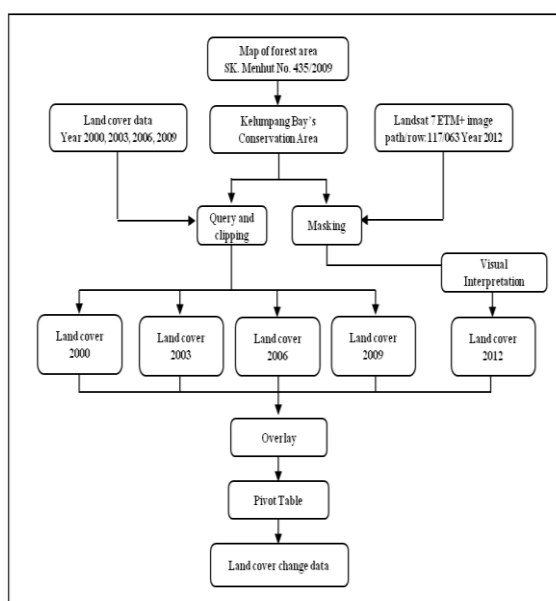
Fig. 1. Data processing.
